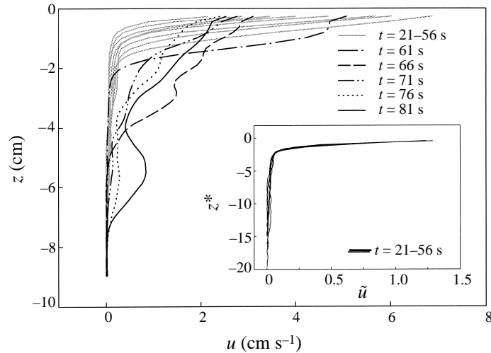
FIGURE 7. Horizontal velocity profiles, for a final wind speed of 3 \text{ m s}^{-1} , obtained by averaging across images comparable to those in figure 6 for a period of 1 s. Up to 56 s the profiles correspond to a monotonically accelerating and deepening shear layer. From 61 s to 81 s the surface velocity decreases as the momentum mixes down to a depth of 8 cm. The inset shows the data from t = 21\text{--}56 s, plotted as \tilde{u} = u/u(z^* = 0.59) versus z^* = z/(vt)^{1/2} . The value of the normalized depth z^* = 0.59 was chosen as the minimum depth (2.7 mm) at the minimum time (21 s) for this sequence.
